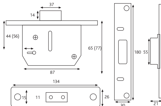
5 Lever Deadlock
