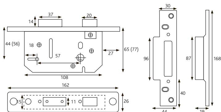
5 Lever Sashlock
