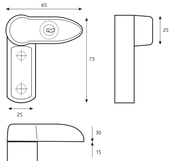
Keyed Snaplock
