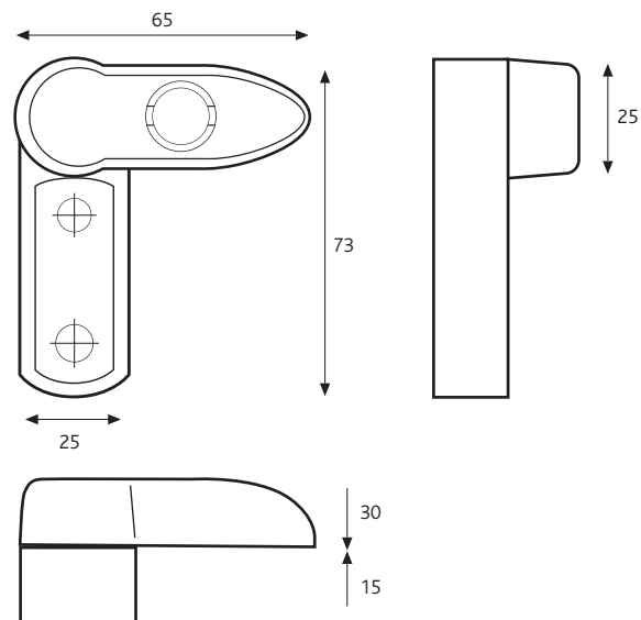
Keyless Snaplock
