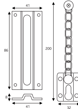
Slide Chain
